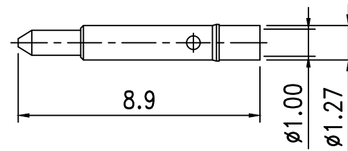
RECOMMENDED USE CRIMP TOOL DIE 0.213"
