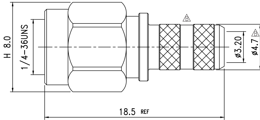
RECOMMENDED USE CRIMP TOOL DIE 0.213"
