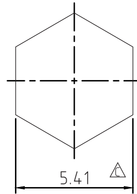
RECOMMENDED USE CRIMP TOOL DIE 0.213"
